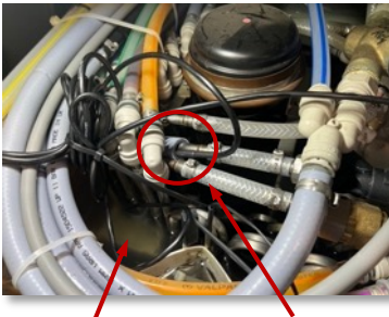
Temperature probe - Ice Bath (Hidden) Temperature probe - Water Flow to Drinks Tower
